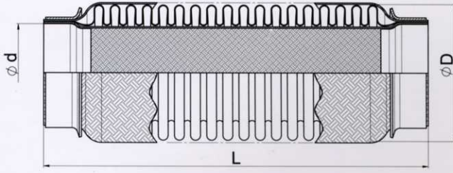
İÇ ÖRGÜLÜ / WITH INNER BRAID
